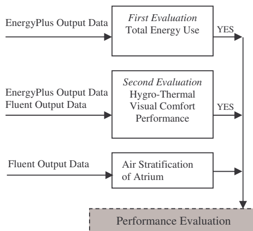
Figure 4 Performance evaluation of atrium
