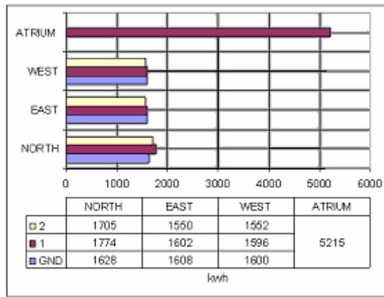
Figure 9 Annual lighting energy consumption of the zones in kWh
