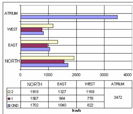
Figure 7 Annual heating energy use of the zones in kWh
