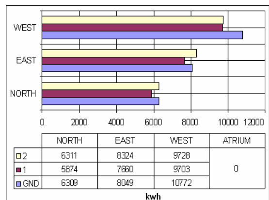
Figure 8 Annual cooling energy consumption of each zone in kWh
