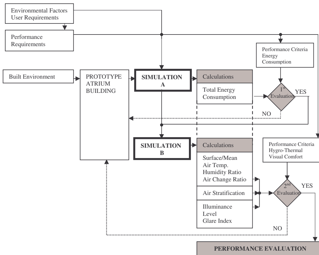
Figure 1 Simulation model for energy performance and user comfort evaluation of atrium buildings
