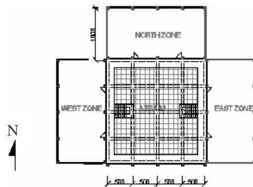
Figure 6 Plan of the office building
